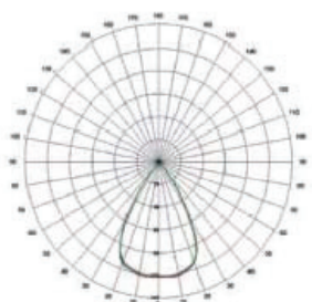
60° light distribution curve
